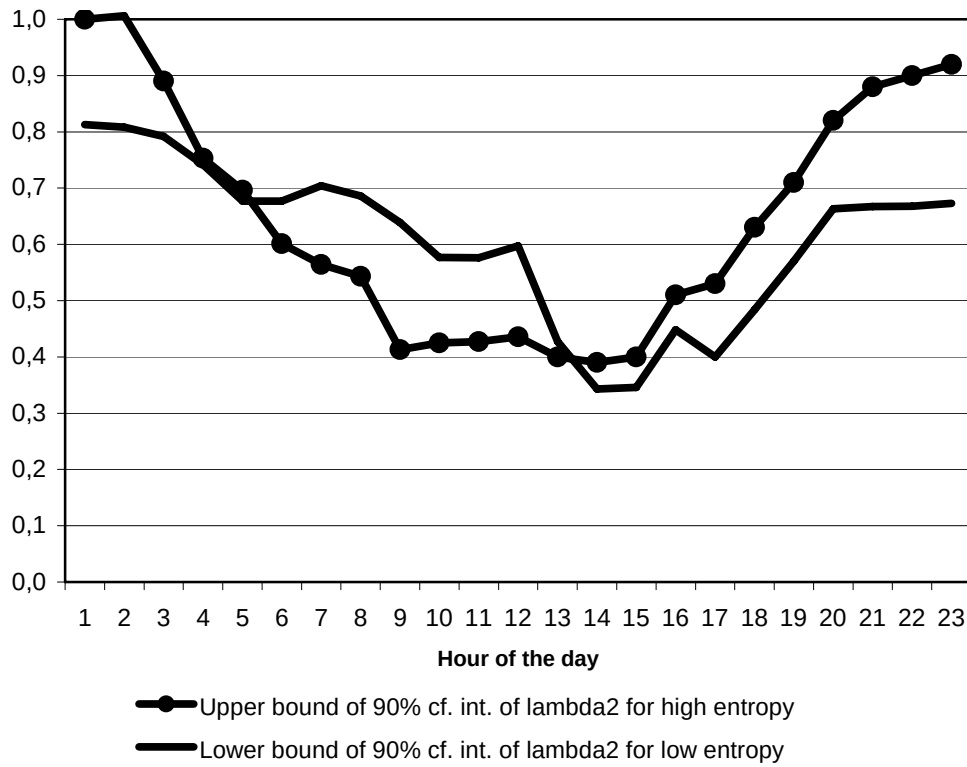
Figure 6 90% asymmetric confidence intervals for \lambda_{2high} and \lambda_{2low}
